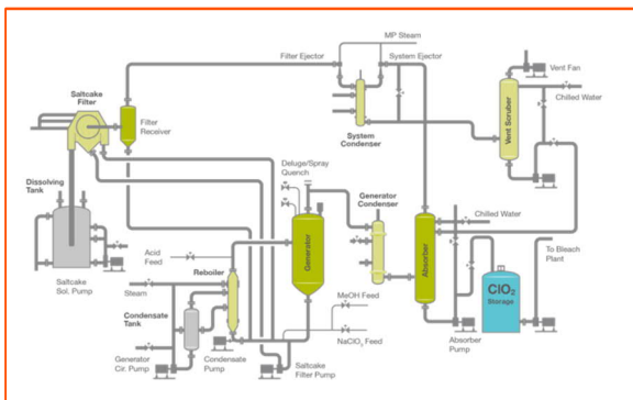
SVP Chlorine Dioxide Generator Process Flow Diagram
